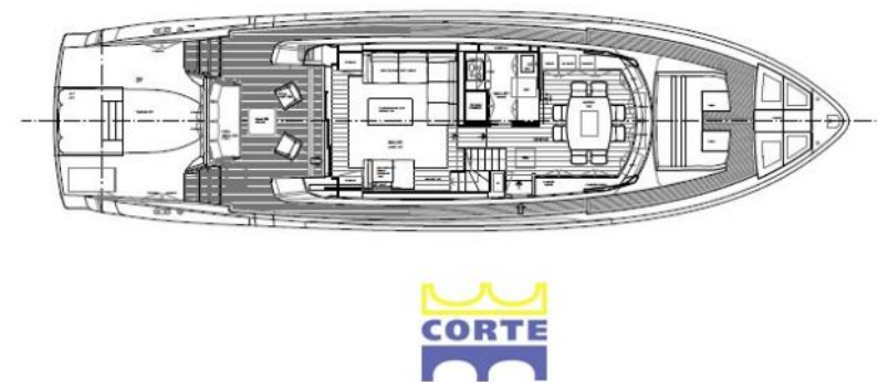
16. General arrangement plans
