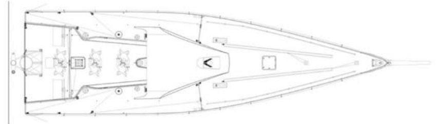
DECK LAYOUT
